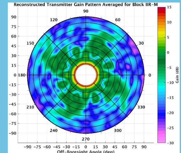
Block IIR-M reconstructed pattern from GPS ACE [11]
