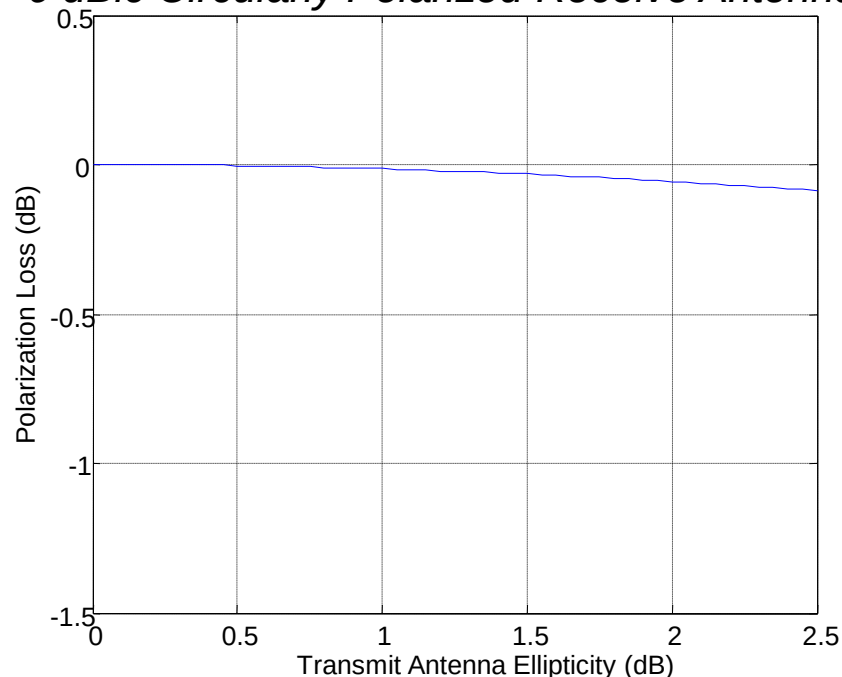
Polarization Loss at Worst Orientation into 0 dB Circularly Polarized Receive Antenna
